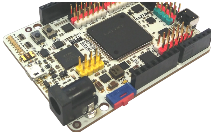
IceZUM Alhambra v.11 open FPGA Board (6 unidades)
